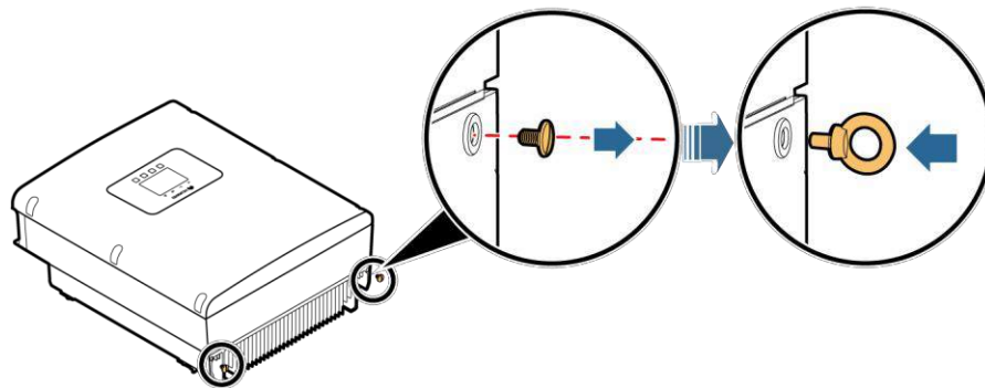
Figure 1-10 Installing lifting eyes
