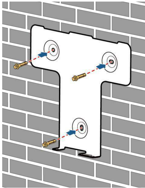
Figure 1-9 Securing a rear panel
