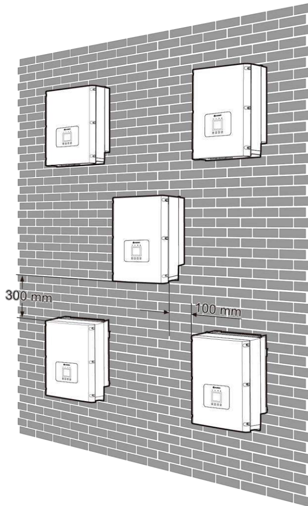
Figure 1-5 Triangle installation mode
