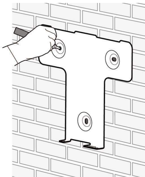
Figure 1-3 Hole positions and dimensions
