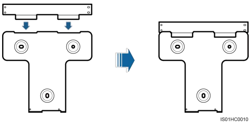
Figure 1-14 Mounting the SUN2000 on the rear panel (rear view)
