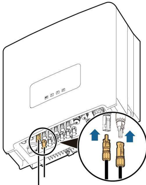
Figure 1-31 Connecting DC input power cables (4)
