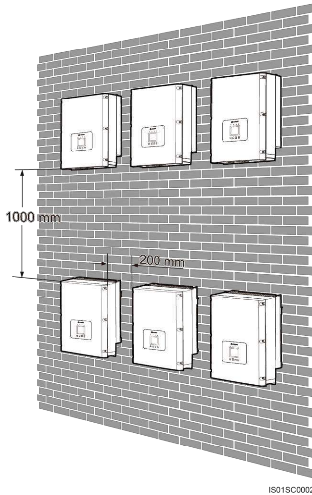
Figure 1-6 Stacked installation mode
