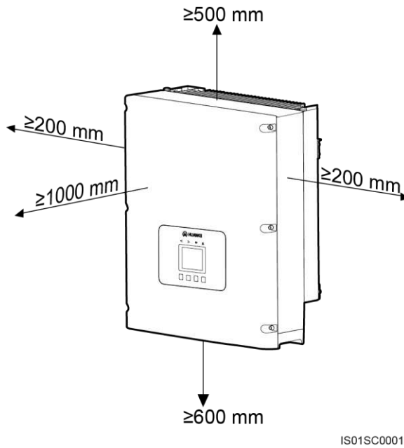
Figure 1-4 Minimum installation clearance
