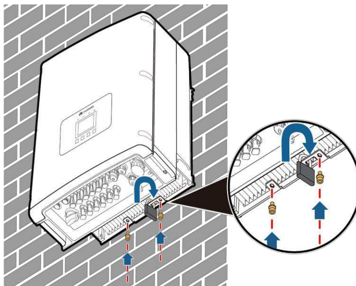
Figure 1-15 Tightening hexagon screws
