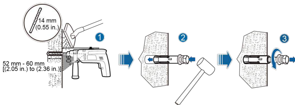
Figure 1-8 Drilling a hole and installing an expansion bolt
