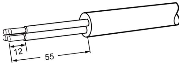
Figure 1-18 Connecting an AC output power cable (1) (unit: mm)
