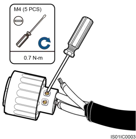
Figure 1-22 Connecting an AC output power cable (5)
