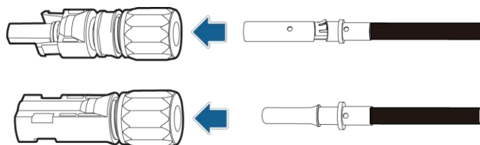
Figure 1-29 Engaging metal terminals
