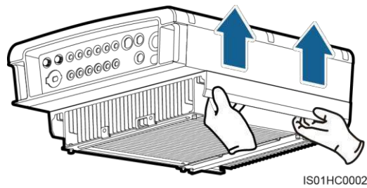
Figure 1-2 Moving the SUN2000 (2)
